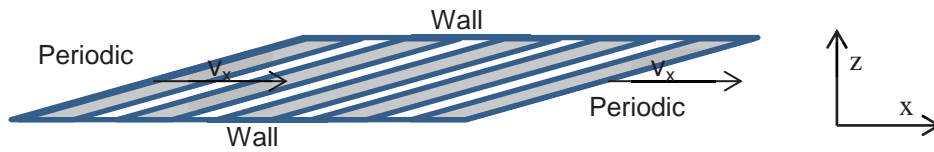
Figure 4. Boundary conditions for the simulation of the EOLE facility
