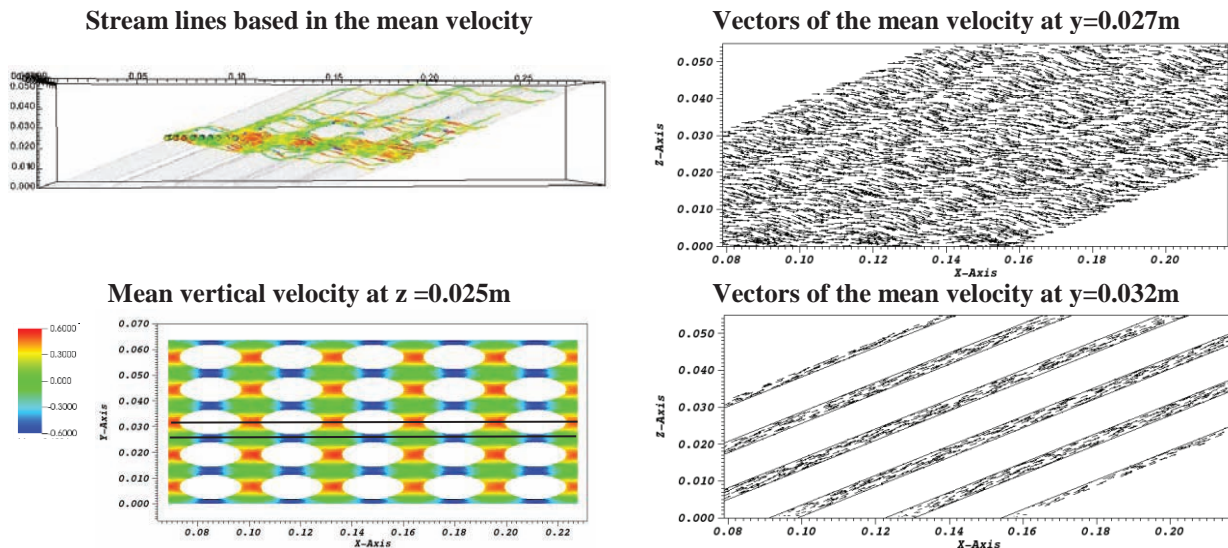
Figure 5. Flow field of the simplified calculation of the EOLE experiment
