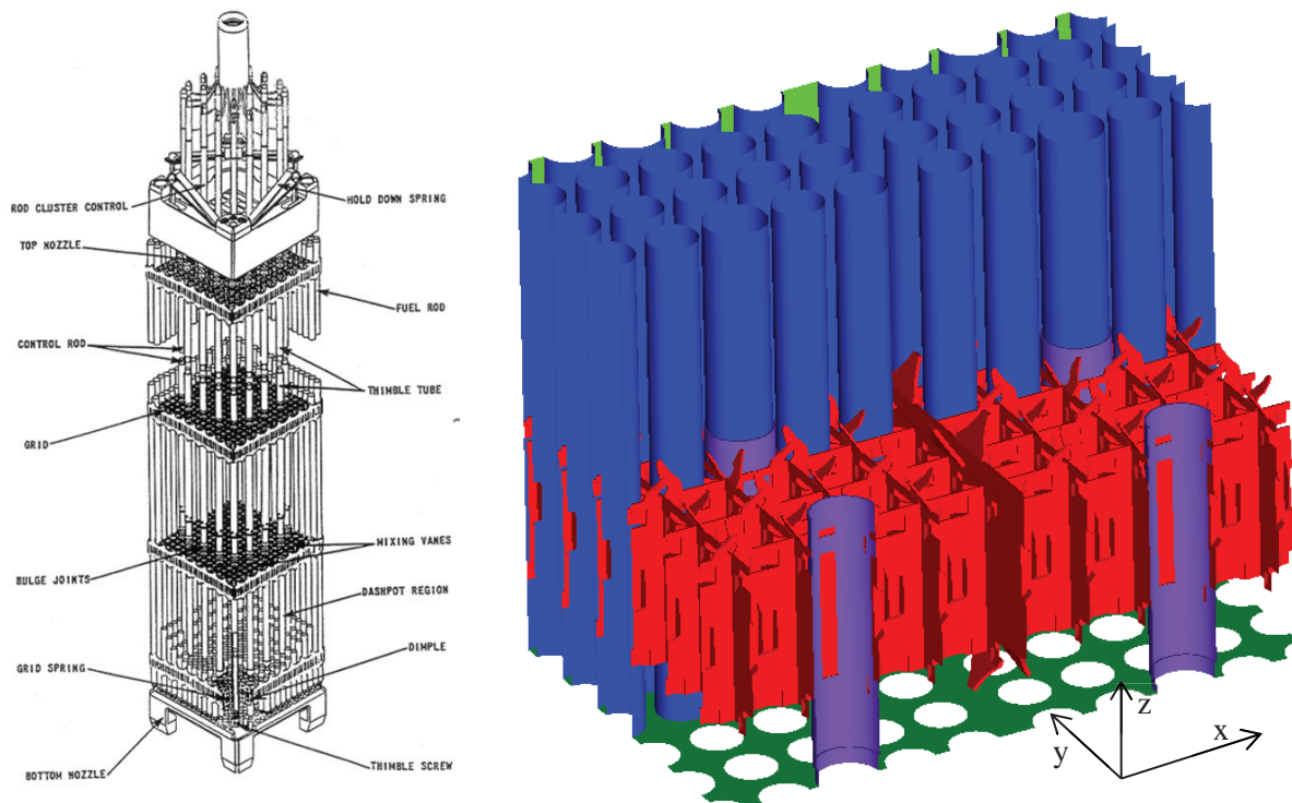
Figure 6. Typical fuel assembly and CAD model of the mixing grid with fuel and control rods
