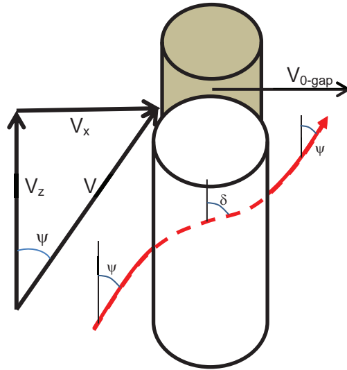
Figure 2. Schematic stream line between two adjunct fuel rods
