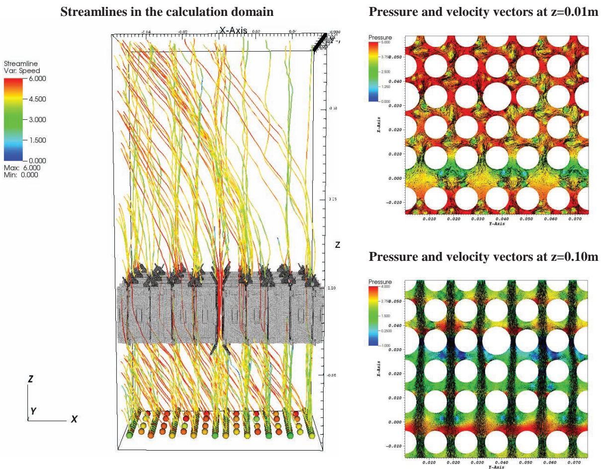
Figure 8. Streamlines as well as reduced pressure and velocity vectors in horizontal cut planes
