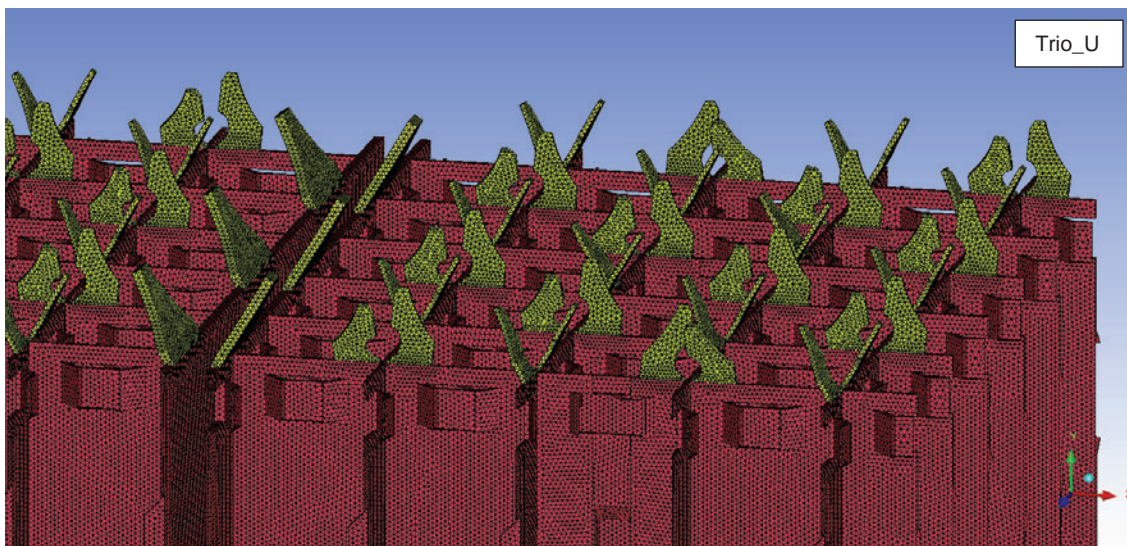
Figure 7. Surface meshing of the mixing grids
