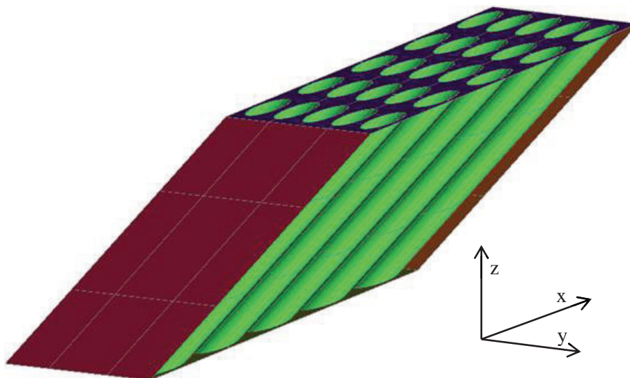
Figure 3. CAD model for the simplified EOLE geometry
