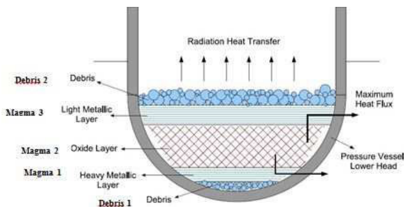
Figure 1. A typical debris configuration in lower plenum.
