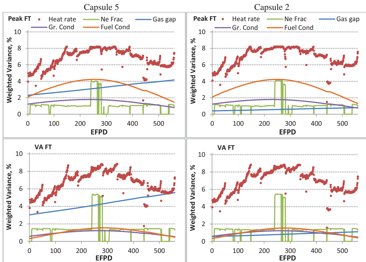
Figure 8. Daily weighted temperature variances due to parameter uncertainties.
