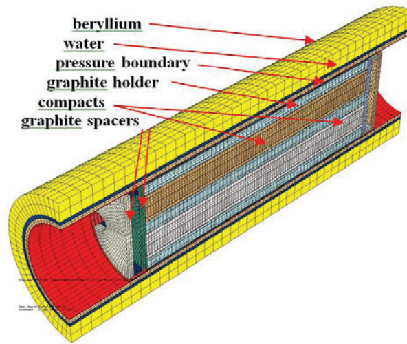
Figure 1. Sideways cutaway view of mesh for an AGR capsule.
