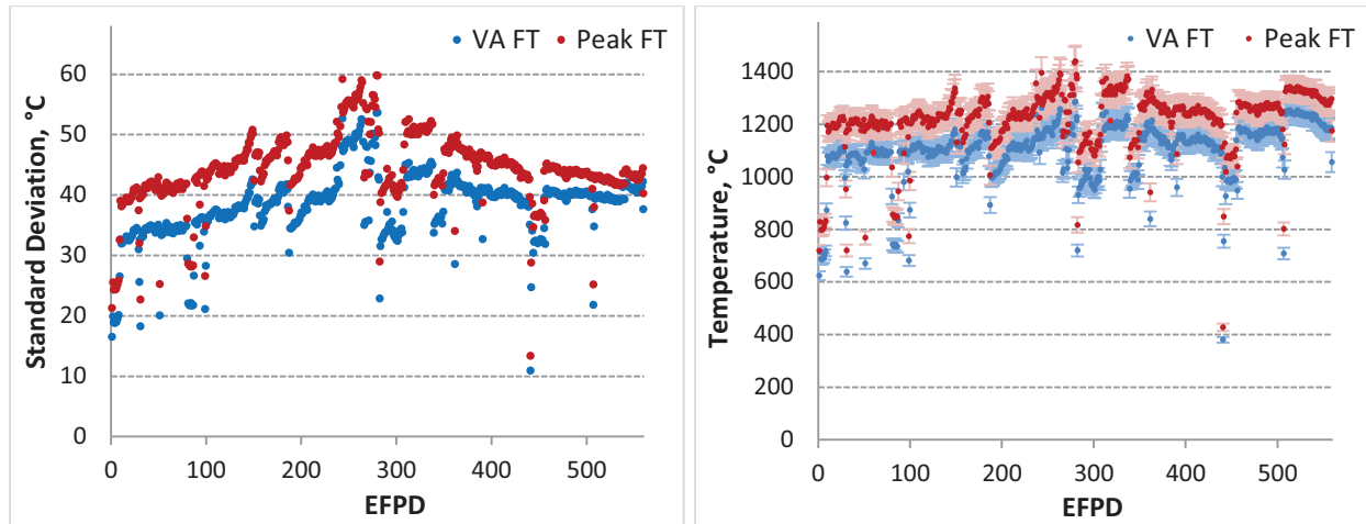
Figure 9. AGR-2 Capsule 5 VA and peak fuel temperature daily uncertainties: Left – uncertainty in terms of standard deviation; Right - temperatures and uncertainty bars.
