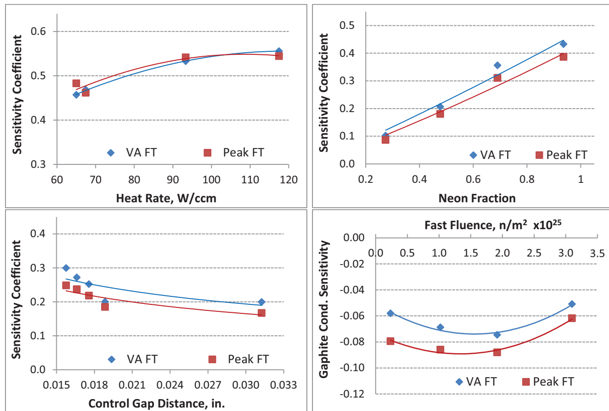
Figure 5. Sensitivities for peak and average (VA) fuel temperatures as function of input.
