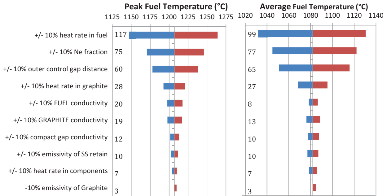
Figure 3. Sensitivities for peak and volume-average fuel temperatures.
