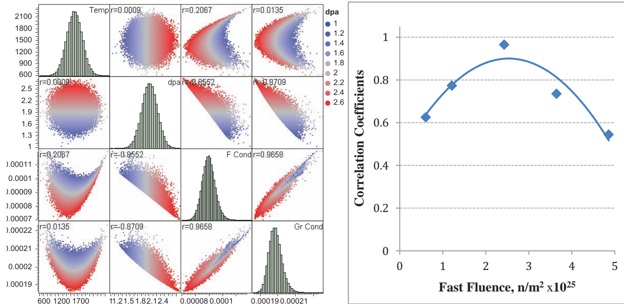
Figure 7. Scatter plot matrix shows the correlation between fuel and graphite thermal conductivities (left) and correlations as function of fluence (right).
