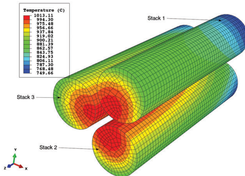
Figure 2. Temperature distribution in cutaway view of three fuel stacks.
