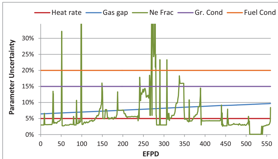
Figure 6. AGR-2 Capsule 5 parameter uncertainties in terms of relative standard deviation.
