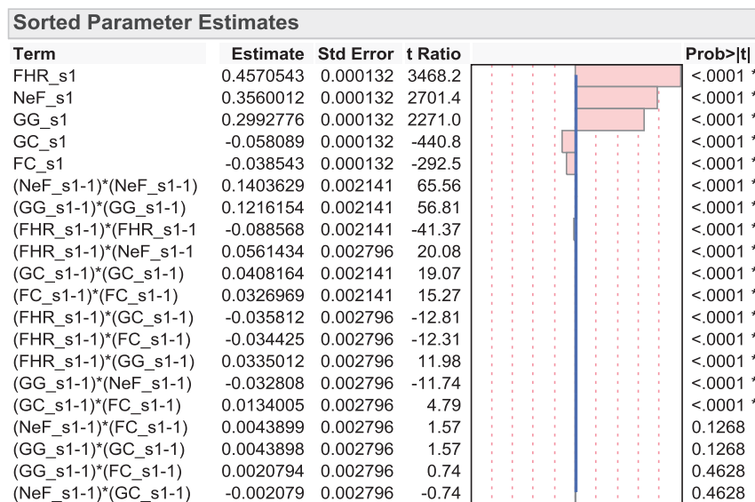
Figure 4. Sorted parameter estimates (Eq. 3) for average fuel temperature.
